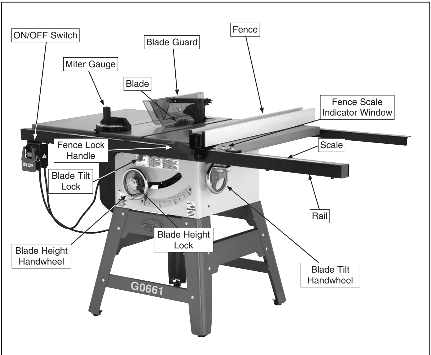
Figure 1. G0661 Identification.
